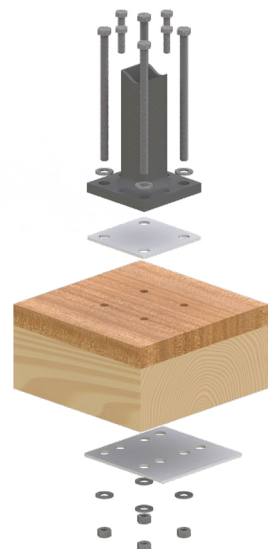
NEWELMOUNT-W POST MOUNT HARDWARE KIT FOR WOOD APPLICATION
