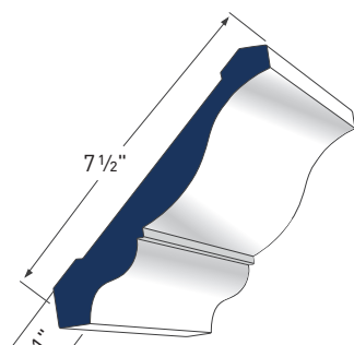
8" CROWN AZM-43 LENGTH: 16'
