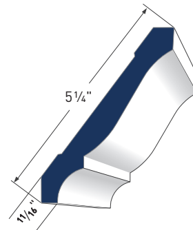
6" CROWN AZM-45 LENGTH: 16'
