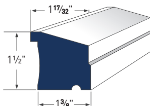
SUB SILL NOSE AZM-6933
