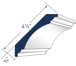
COVE MOULDING AZM-80 LENGTH: 16'
