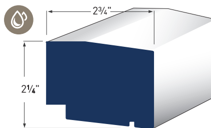
FARMHOUSE SILL AZM-7640
