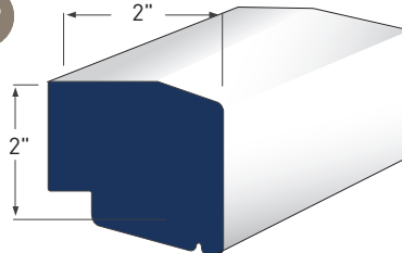
LARGE SILL NOSE AZM-7979
