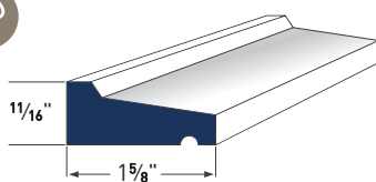
DRIP CAP AZM-197
