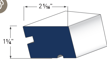
WINDOW SILL NOSE AZM-7974
