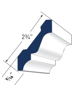
3" CROWN AZM-52 LENGTH: 16'
