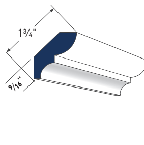
BED MOULDING AZM-75 LENGTH: 16'
