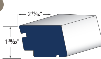
LARGE HISTORIC SILL AZM-7958
